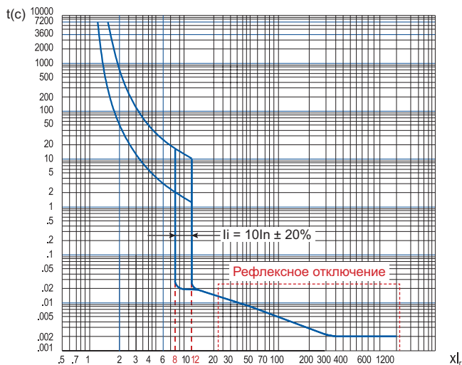
NM8N-125 (80, 100, 125 A)
