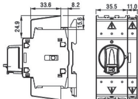
NF2-40/TS
