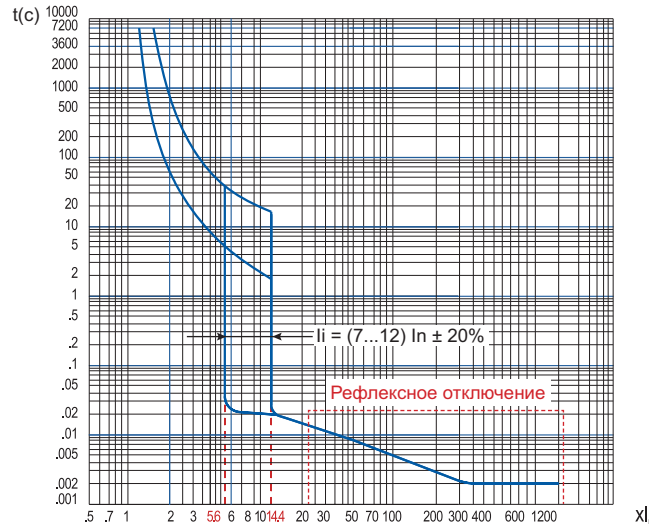
NM8N-250 (125, 160 A)
