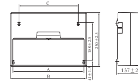
Fig. 1 Single row overall and mounting dimensions
