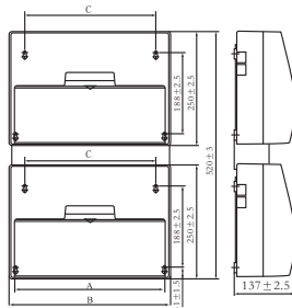
Fig. 2 Double rows overall and mounting dimensions
